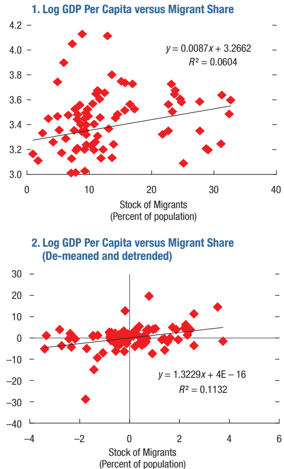
Figure 4. Simple Correlations
