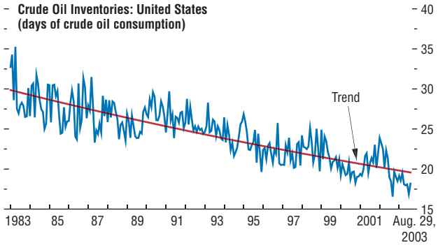
Figure 1.20. Oil Inventories
