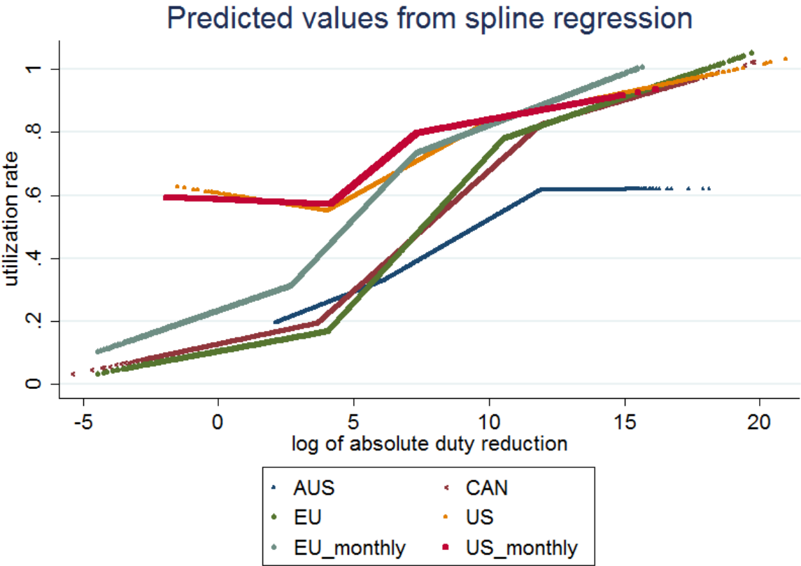
Figure 9: Spline regressions
