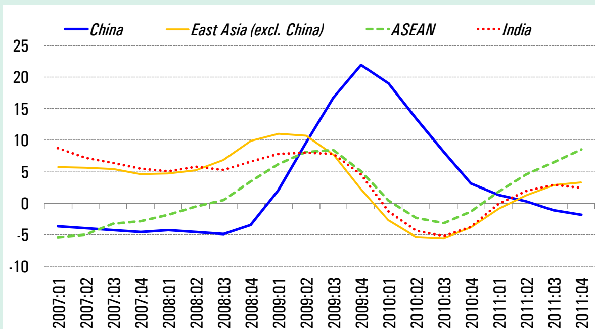
Figure 1.7. Emerging Asia: Measure of Excess Credit Growth 1 (In percentage points; four-quarter moving average)
