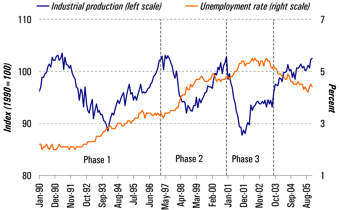
Figure 2.2. Japan: Industrial Production and Unemployment
