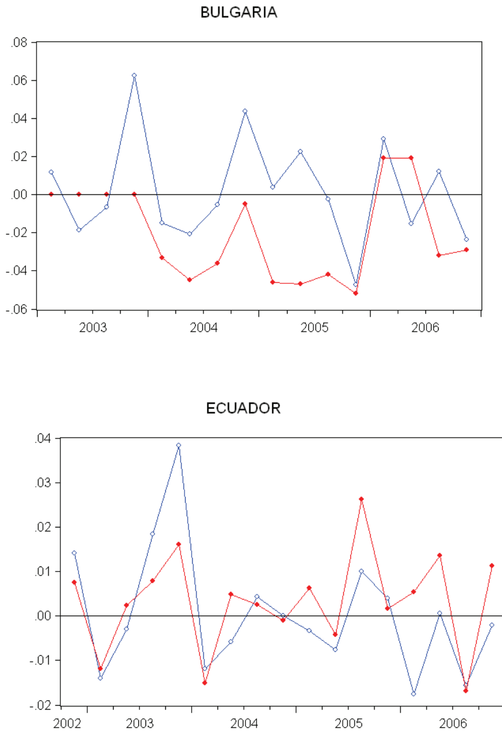
Figure 3a: Central bank estimation errors and VAR residuals
