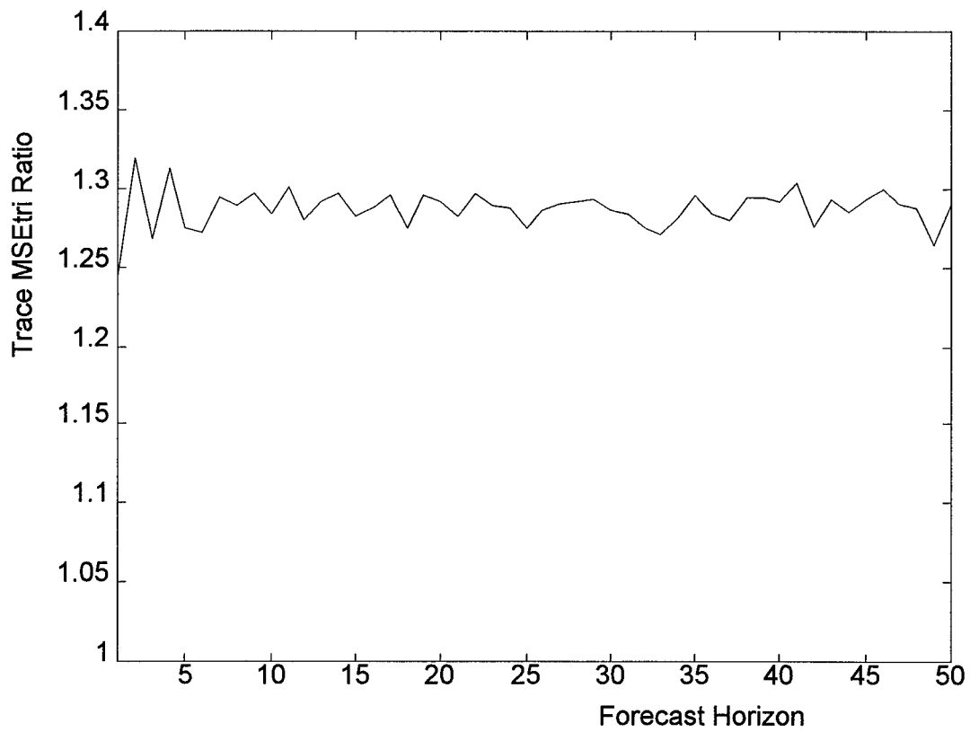
Figure 6 Trace MSE_{tri} Ratio Differenced VAR vs. Cointegrated System Forecasts, Estimated Parameters Bivariate Example, \lambda=q=1
