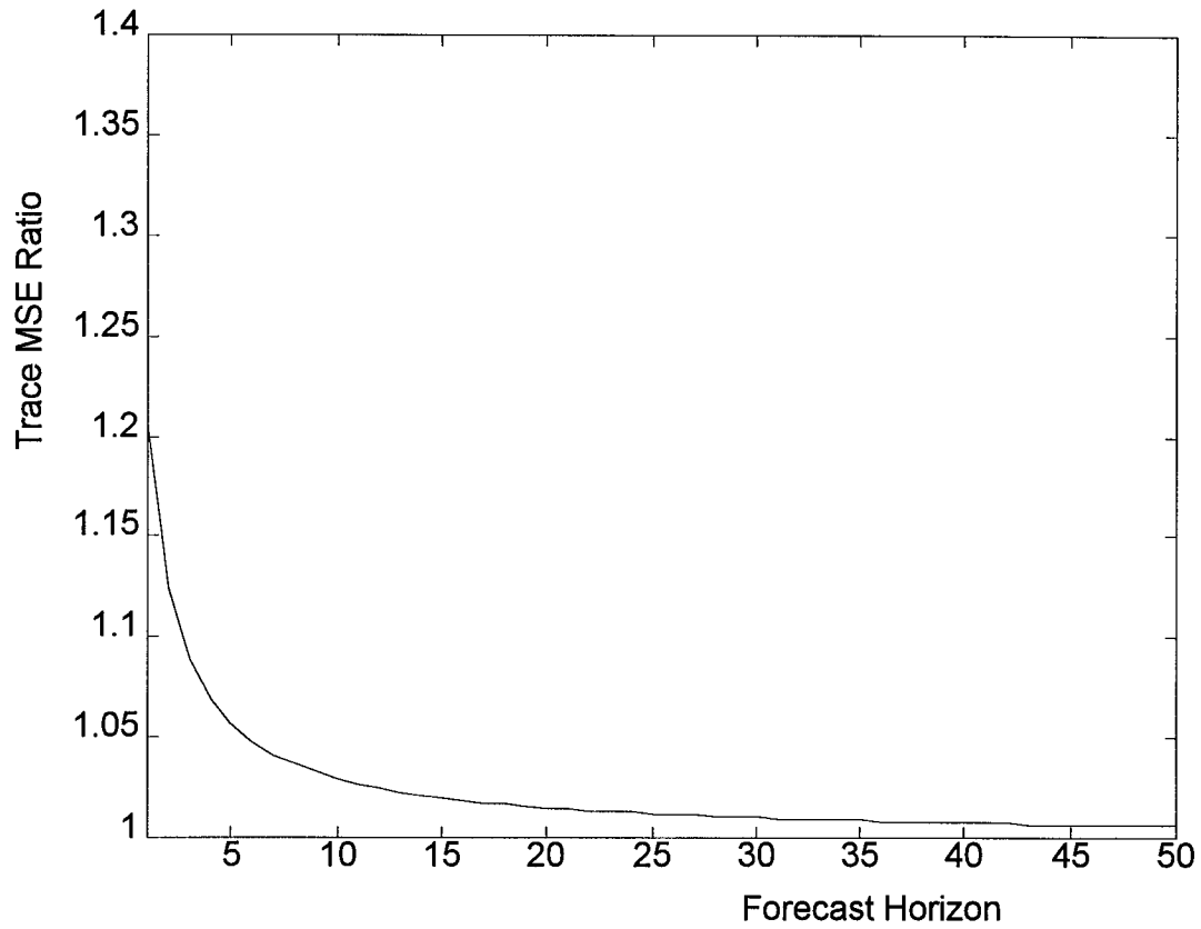
Figure 1 Trace MSE Ratio Univariate vs. System Forecasts Bivariate Example, \lambda=q=1
