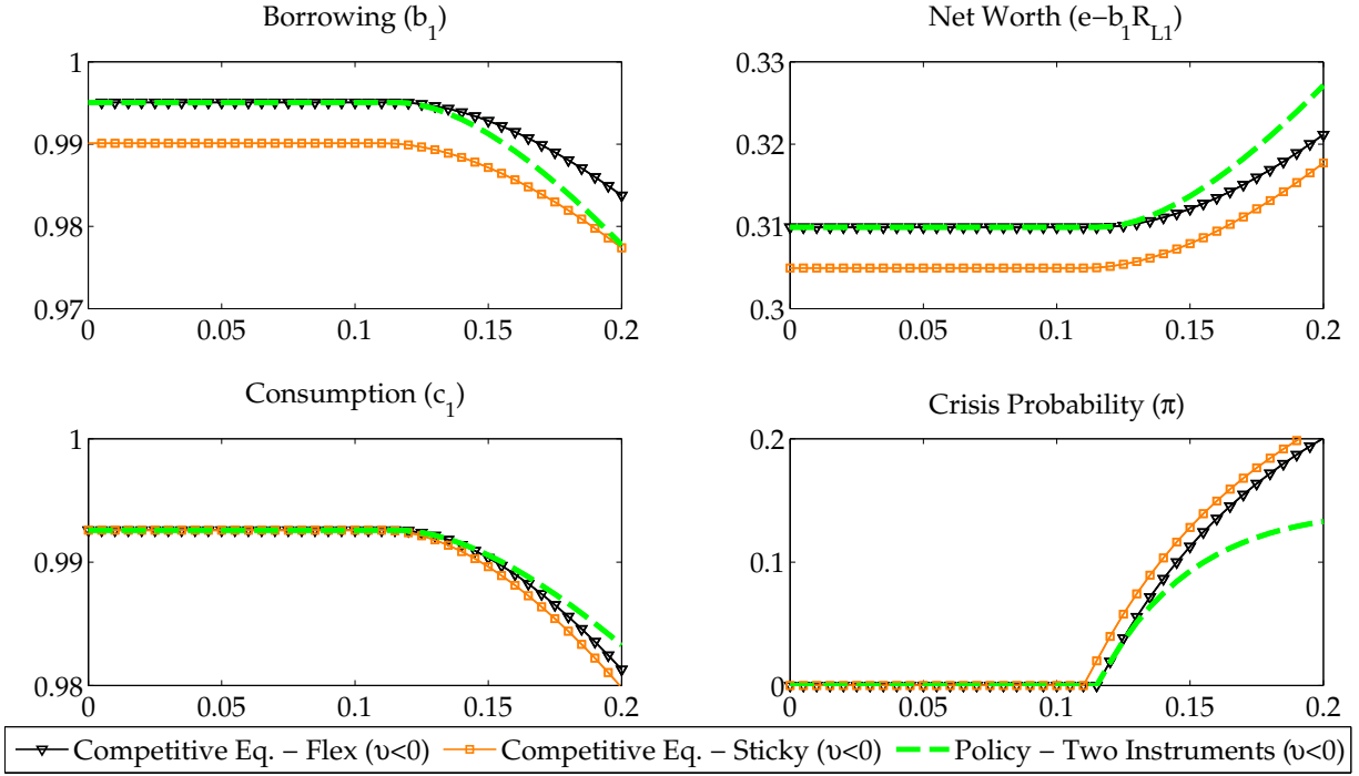
Figure 6 EFFICIENT ALLOCATION WITH BOTH FRICTIONS: NEGATIVE SHOCK TO THE INTEREST RATE. On the horizontal axis is the maximum size of the endowment shock ( \epsilon ). The thin lines with triangle and square markers display the equilibrium after a negative shock hits the risk-free rate under flex-rates and sticky rates, respectively; the dashed line displays the efficient allocation with two policy instruments. A subsidy is in place to remove the distortional effect of monopolistic competition.
