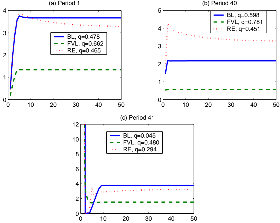
Figure 10: Excess Returns
