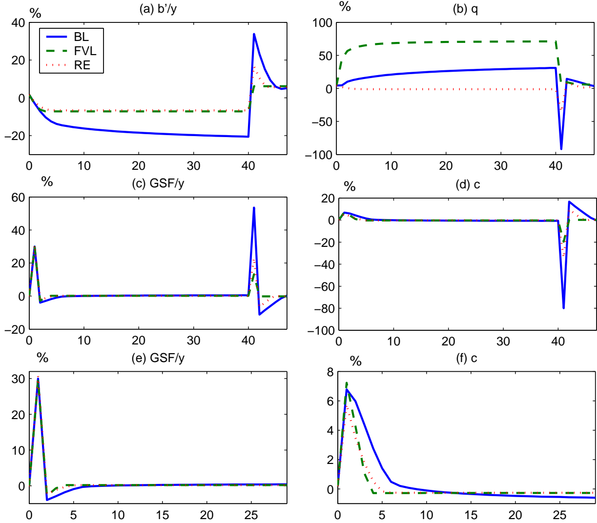
Figure 8: Forecast Functions
