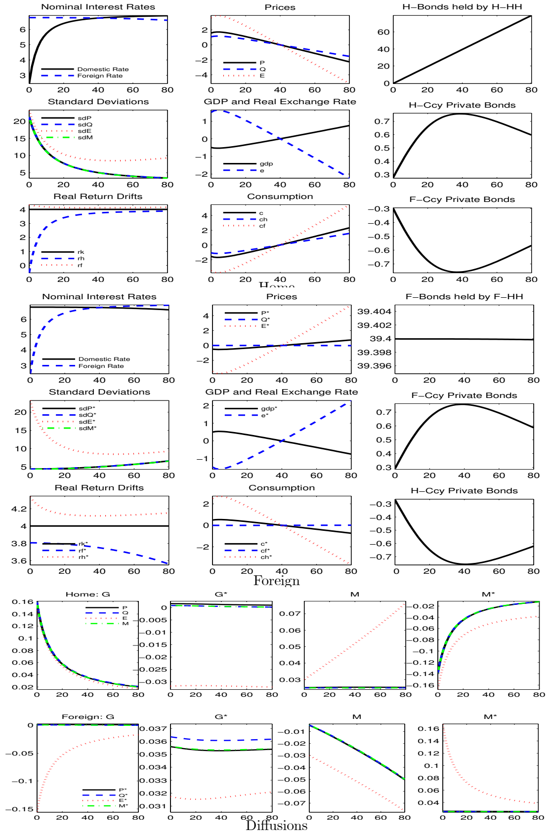
Figure 5. Effects of Government Debt, \phi = \phi^* = 1
