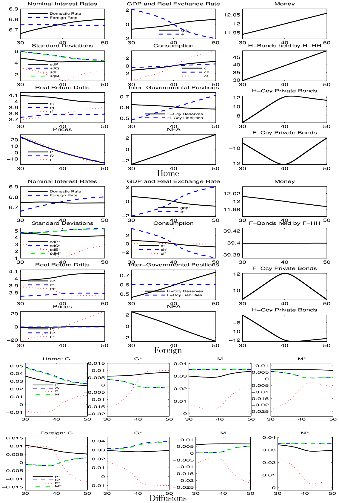
Figure 7. Home Open Market Operations, \phi = \phi^* = 0
