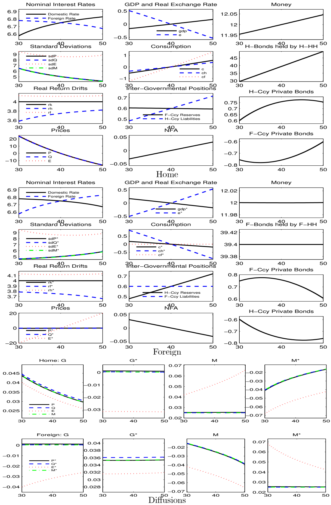
Figure 6. Home Open Market Operations, \phi = \phi^* = 1
