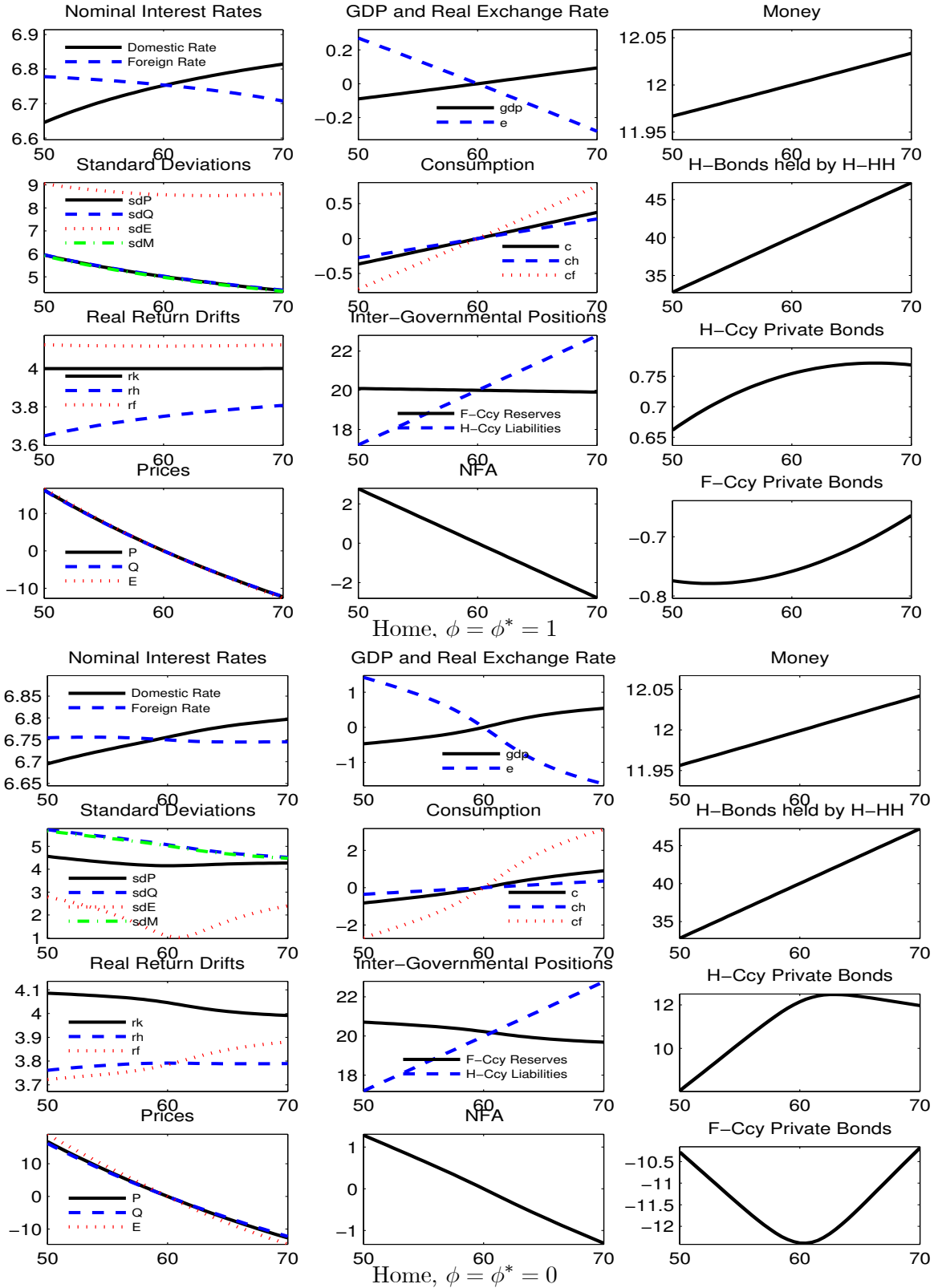
Figure 8. Home Open Market Operations, Large Gross FX Positions
