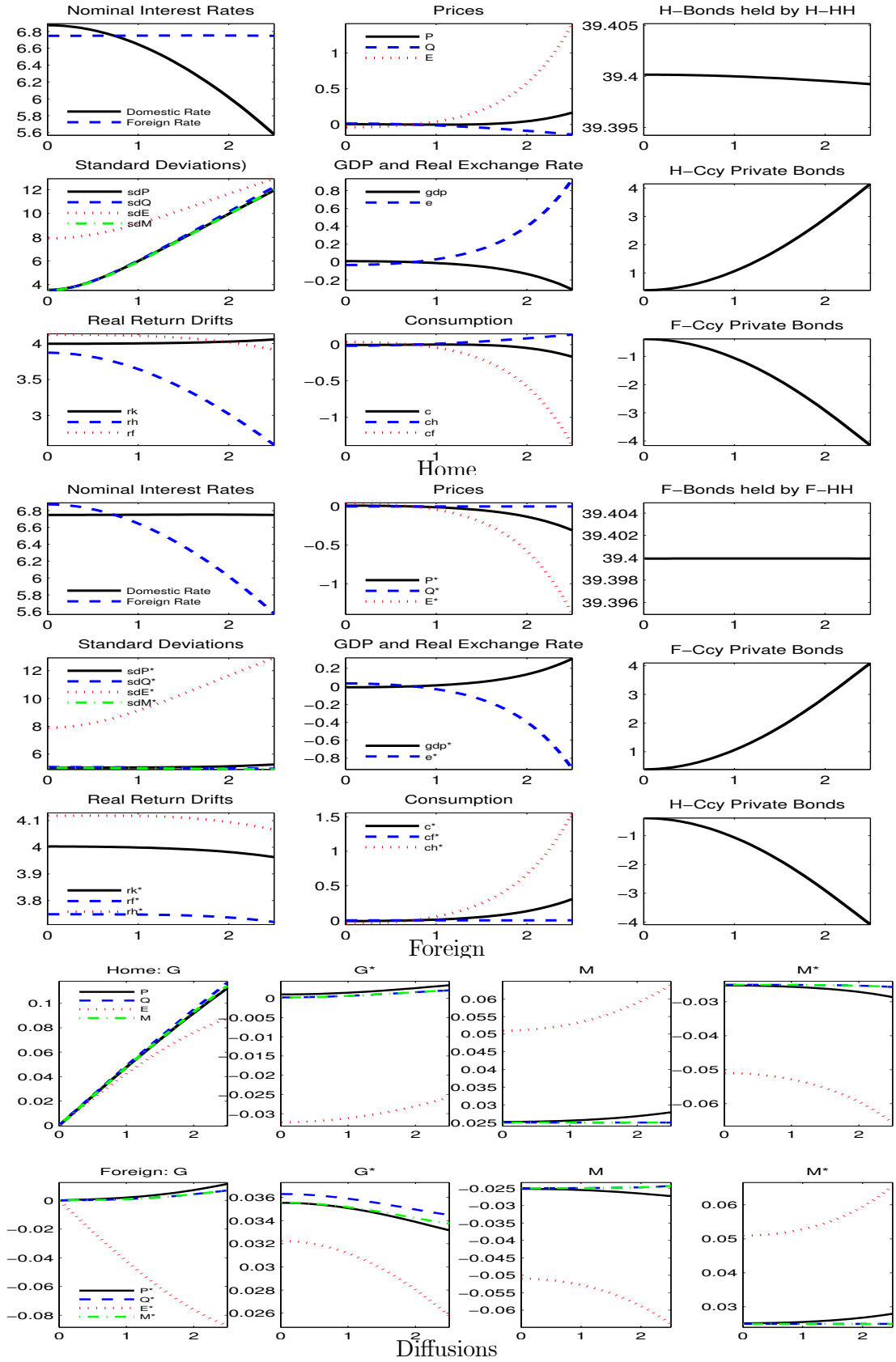
Figure 4. Effects of Government Spending Volatility, \phi = \phi^* = 1
