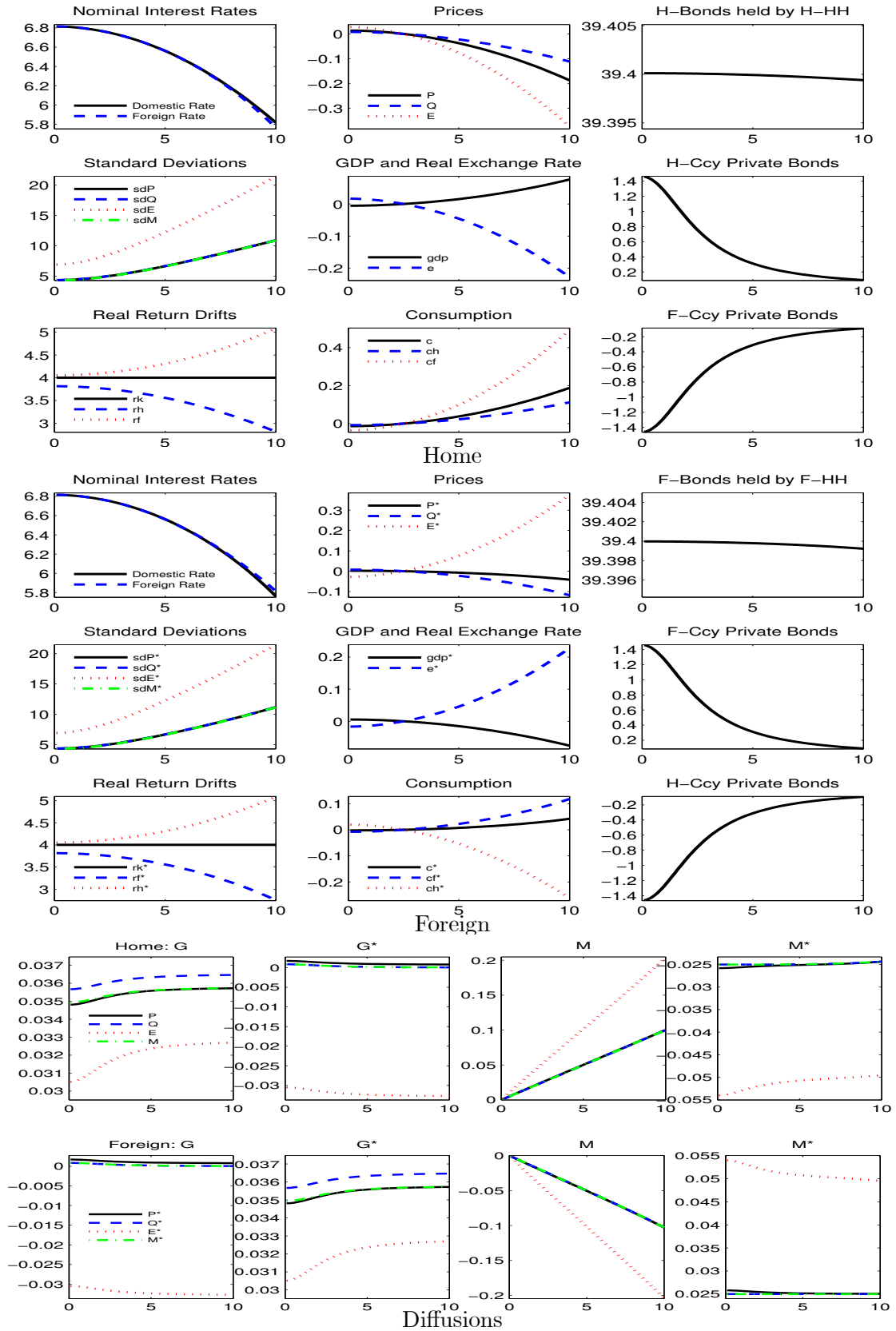
Figure 2. Effects of Money Supply Volatility, \phi = \phi^* = 1
