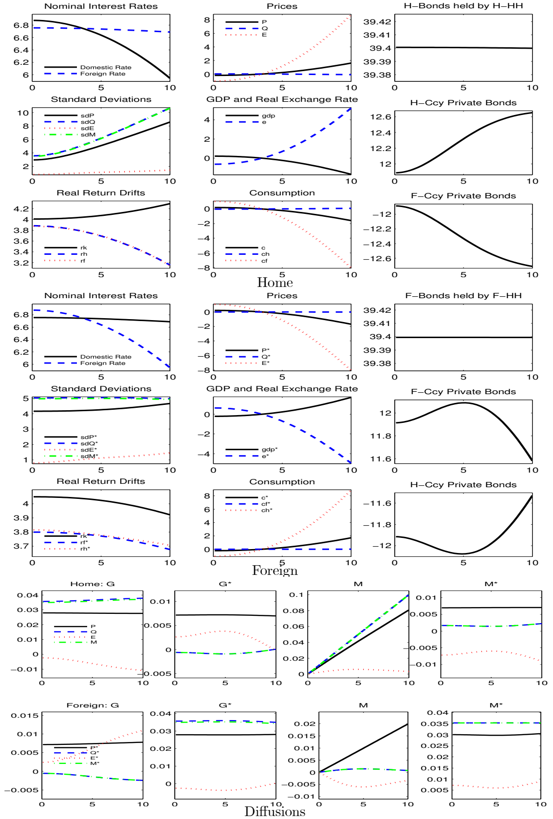
Figure 3. Effects of Money Supply Volatility, \phi = \phi^* = 0
