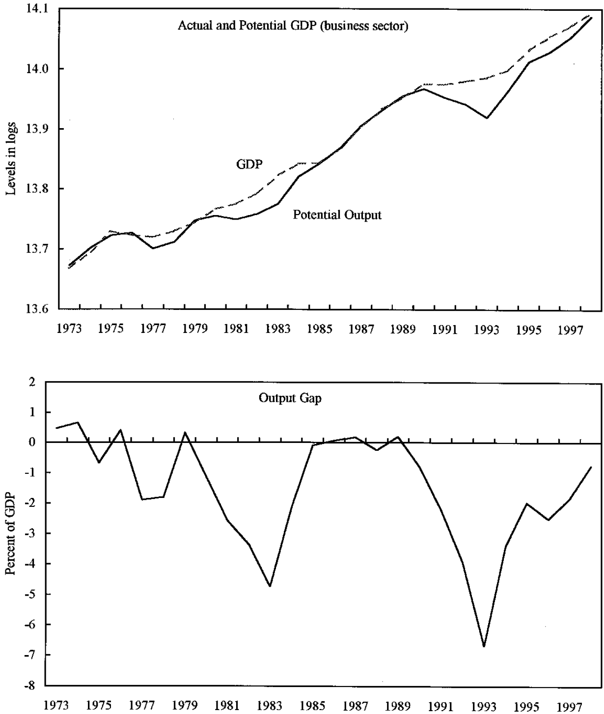
Figure 7. Sweden: Potential Output and Output Gap Production Function Approach
