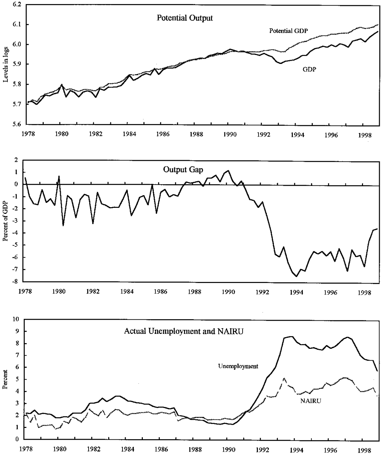
Figure 9. Sweden: Potential Output, Output Gap, and NAIRU System Unobserved Components Method
