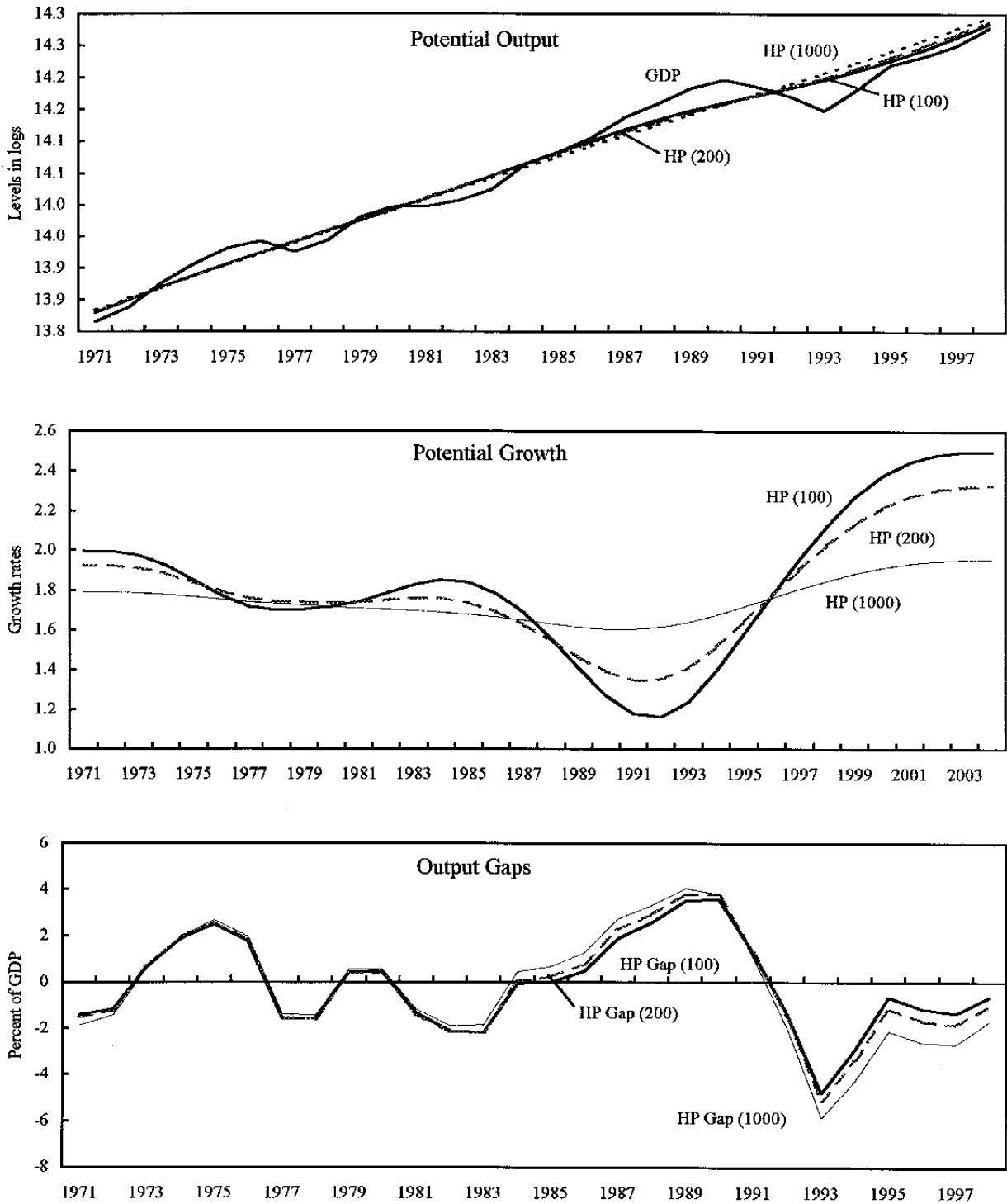
Figure 1. Sweden: Potential Output, Growth, and Output Gaps HP Filter with Smoothing Parameters 100, 200, and 1000
