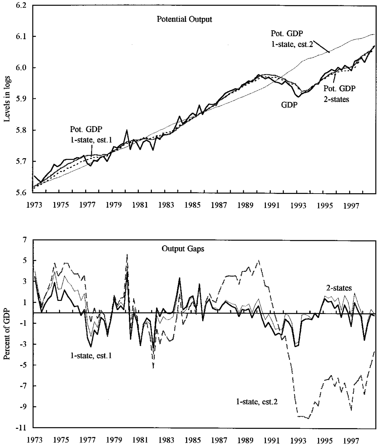
Figure 3. Sweden: Potential Output and Output Gaps Common Permanent and Cyclical Components
