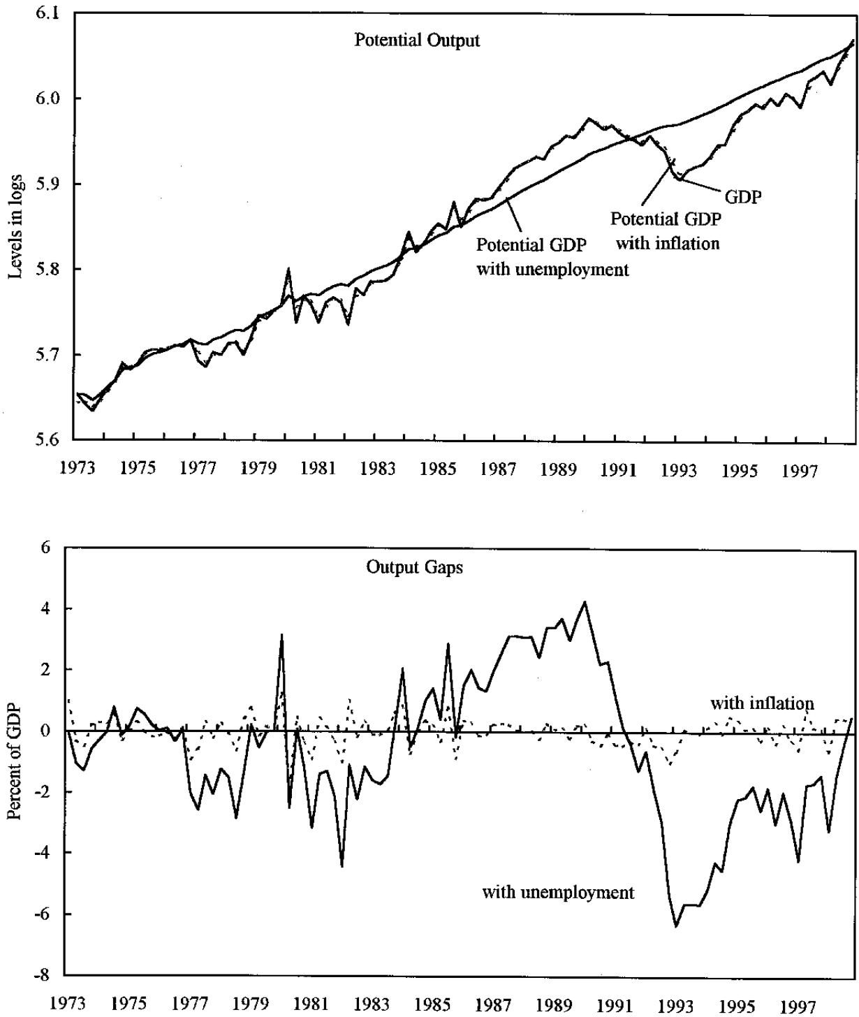
Figure 2. Sweden: Potential Output and Output Gaps Bivariate Unobserved Components Models with Unemployment or Inflation
