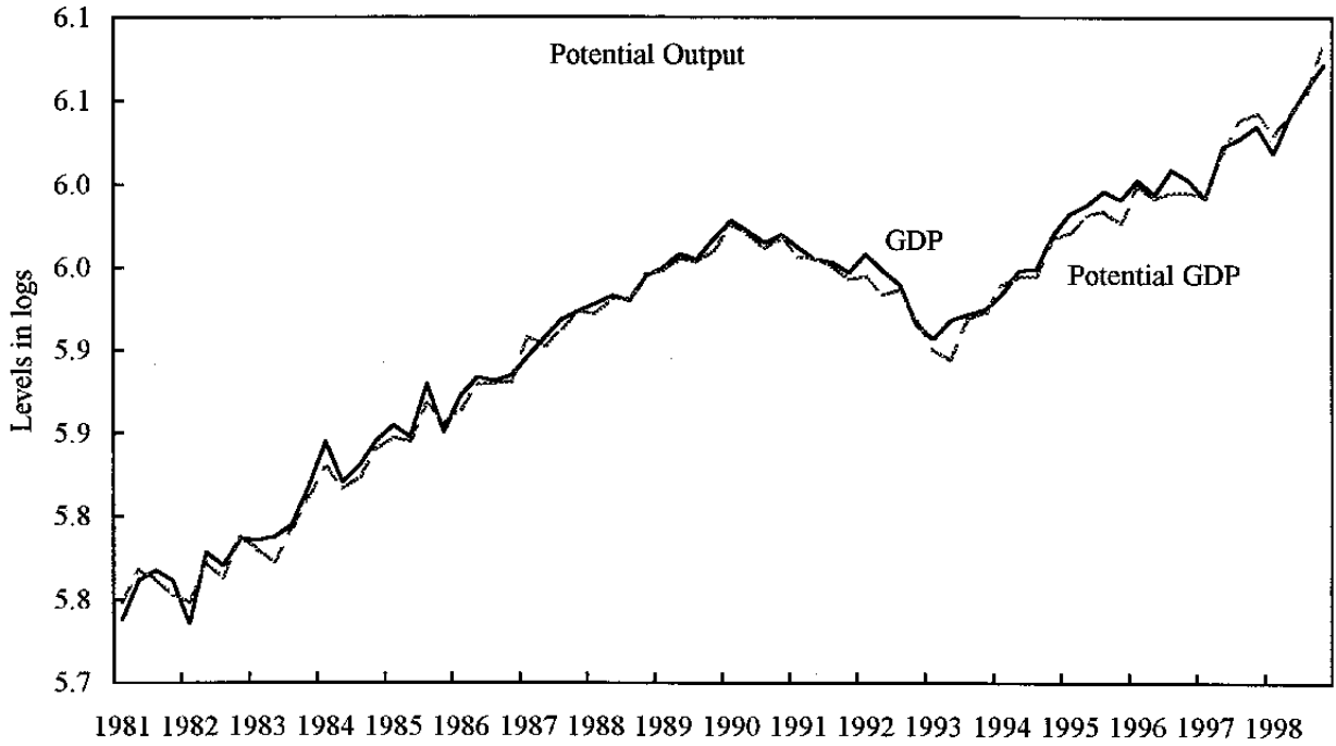
Figure 6. Sweden: Potential Output and Output Gap Structural VAR with Output, Unemployment, and Inflation
