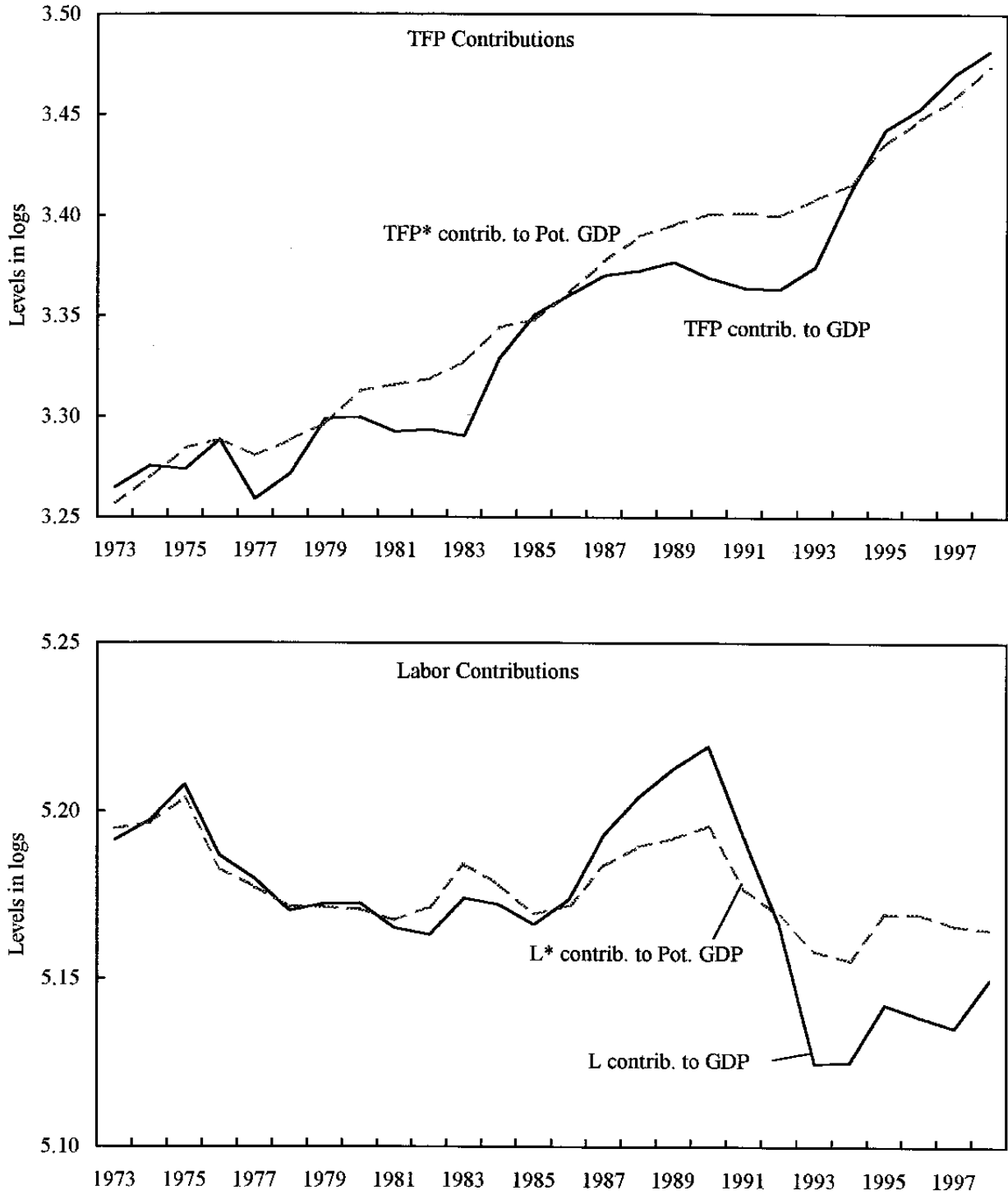
Figure 8. Sweden: TFP and Labor Contributions to the Levels of GDP and Potential GDP Production Function Approach
