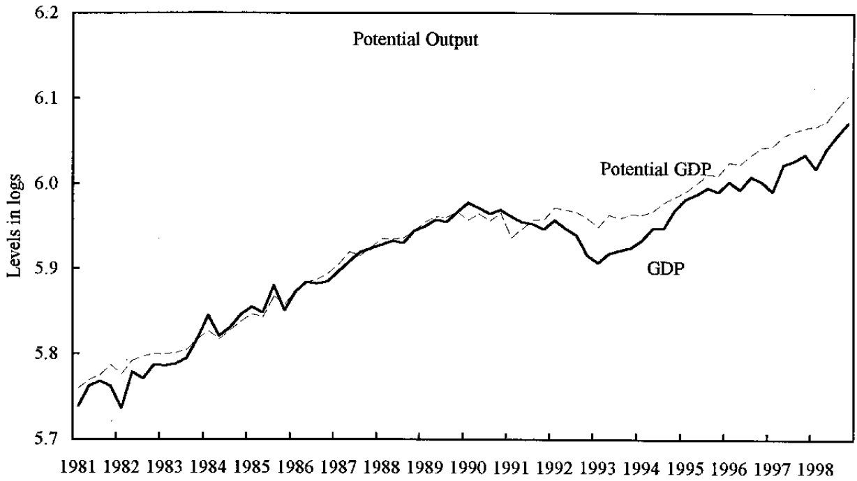
Figure 5. Sweden: Potential Output and Output Gap Structural VAR with Output, the Real Exchange Rate, and Relative Prices
