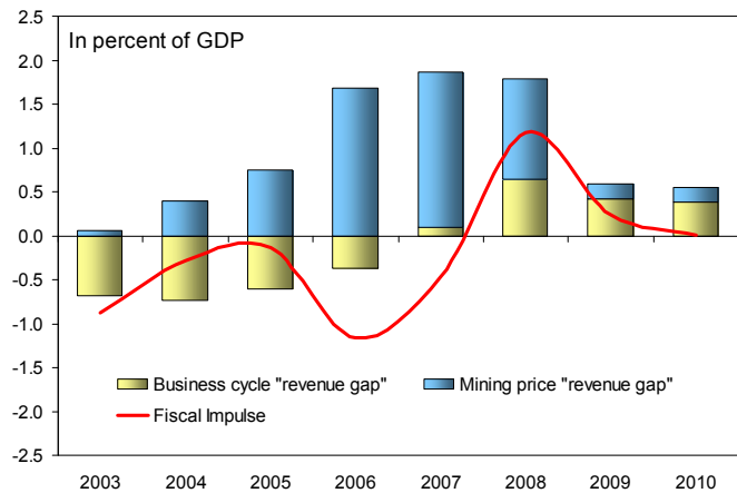
Peru: Structural Fiscal Balance
