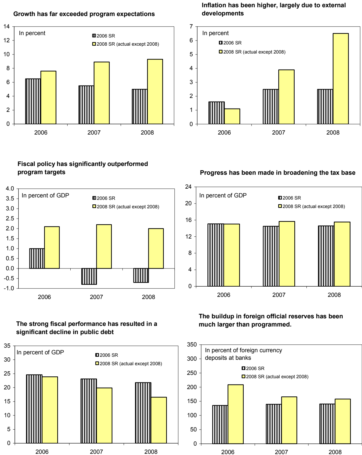
Figure 5. Peru: SBA Objectives and Outcomes, 2006–2008 1/
