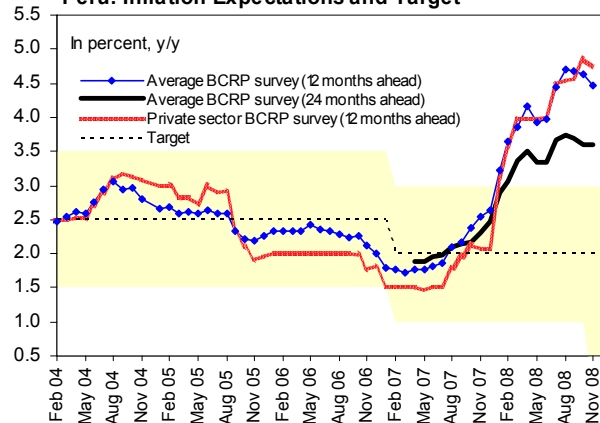
Peru: Inflation Expectations and Target
