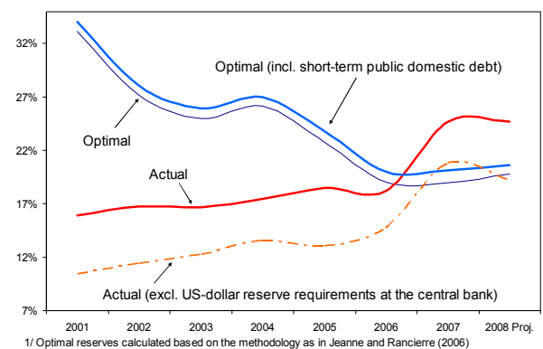
Peru: Official Reserves-to-Output Ratio 1/
