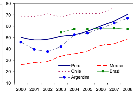
VAT Efficiency for selected Latin American Countries
