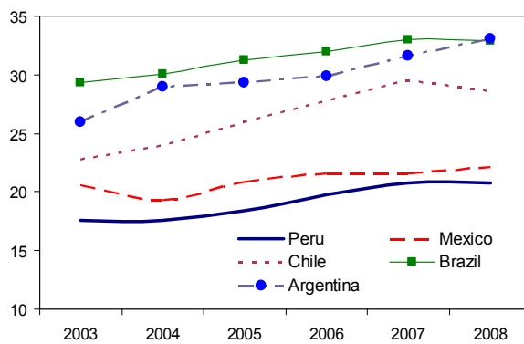
Tax-to-GDP ratio for selected Latin American Countries 1/
