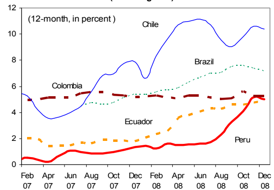
NonTradable Inflation (excluding food)
