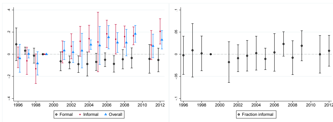
(a) Variance
