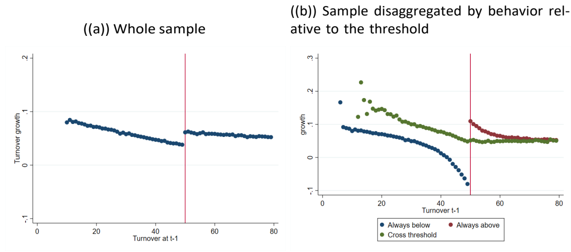
Figure 10. Simulated Data: Turnover Growth
