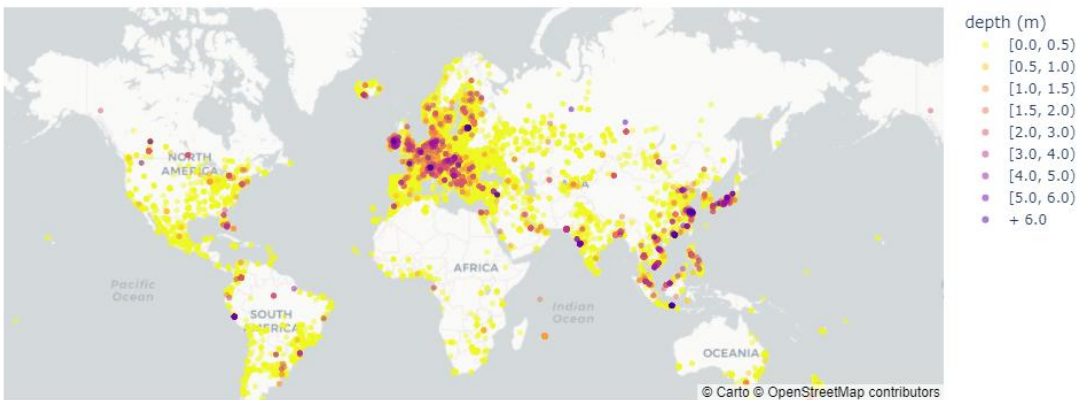
Flood hazard, SSP2 RCP 4.5 1-in-100 year, 2100
