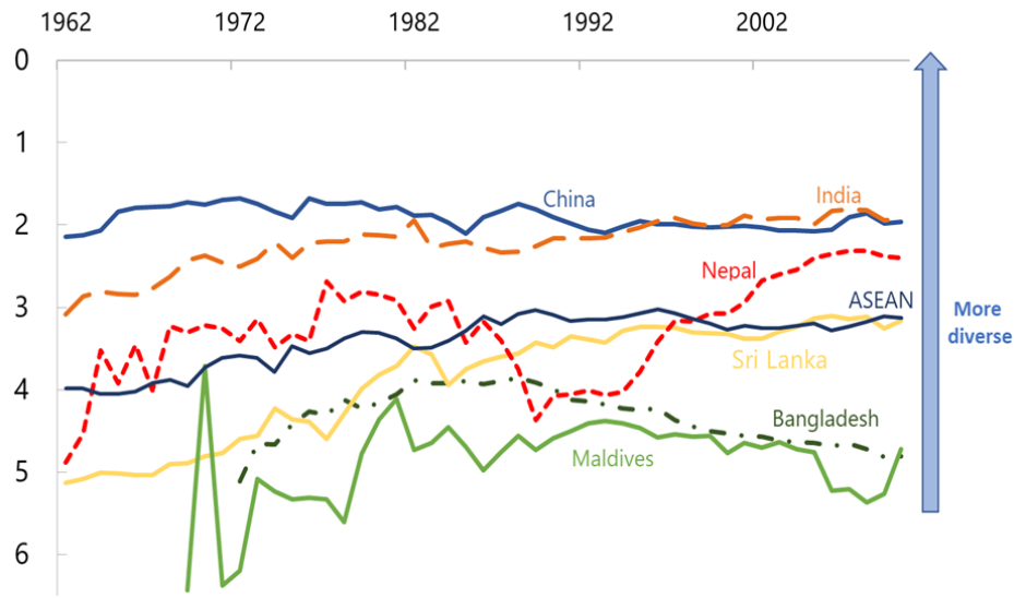
Figure 3. Export Diversification
