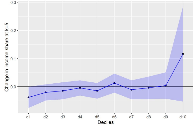
Panel B: Deciles in the income distribution ( k=5 )
